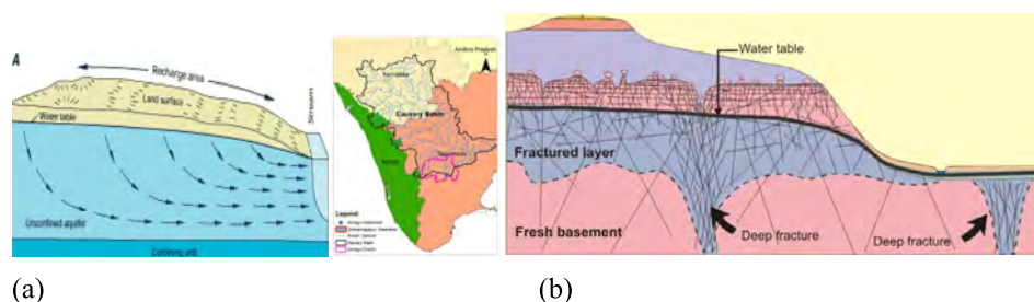
FIGURE 3 (a) Hypothetical situation where ideal homogeneous subsurface geology favours subsurface flow from upstream to downstream. (b) Real situation at Cauvery basin, India, with fractured subsurface layers preventing subsurface flow from upstream to downstream. Source: After Maréchal et al. (2009).
